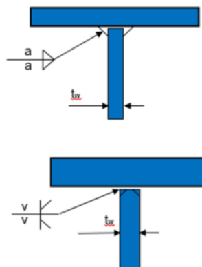
WELD SIZES, I –shape beams and columns
